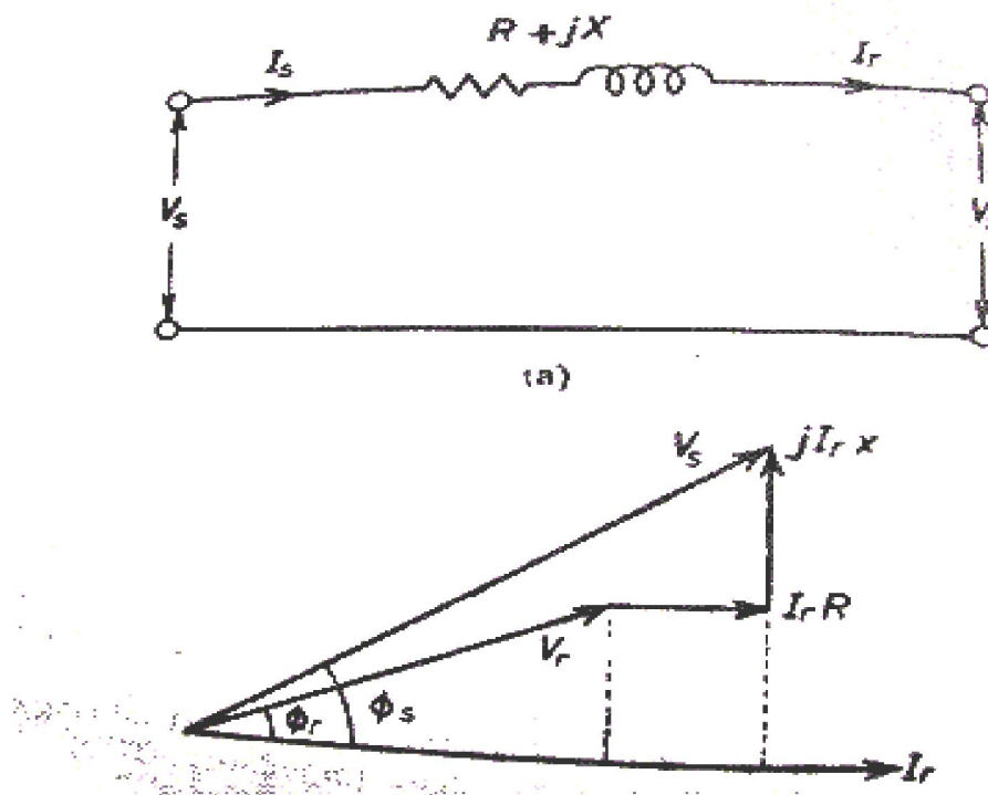
Fig.1.11 Representation of a short transmission line
