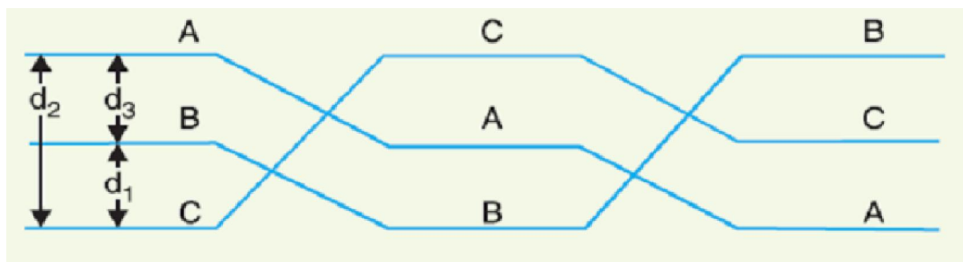
Fig 1.9: Unsymmetrically spaced transposed three phase line
