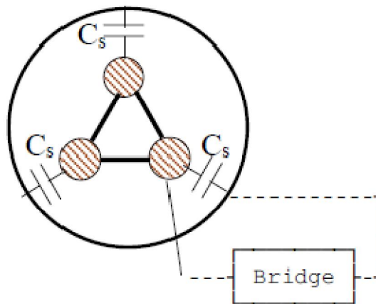
Fig 2.15- Capacitance Measurement
