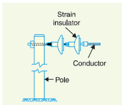
Fig 2.2- Strain Insulator
