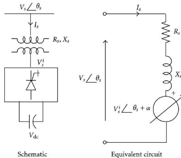
Fig.4.11: Static Synchronous Compensator
