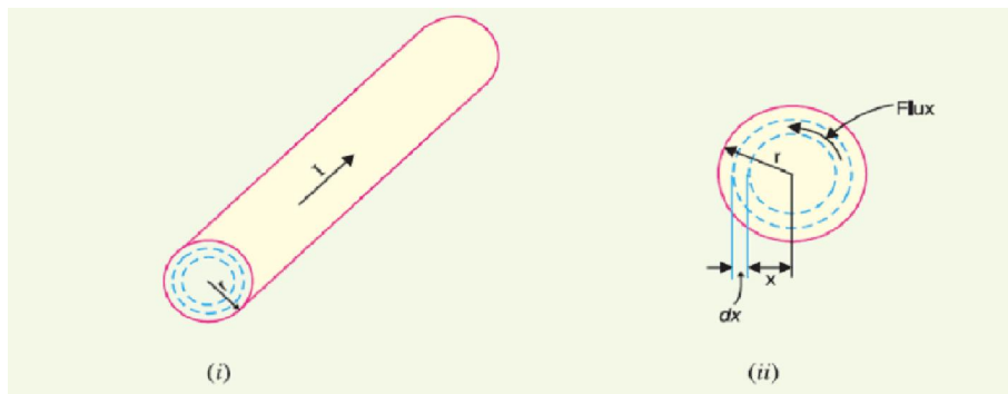
Fig 1.2: Internal flux linkage in a cylindrical conductor
